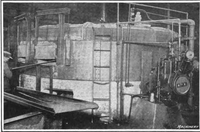
Fig. 33—In the Timken-Detroit Axle Co.'s plant special furnaces with a rotary hearth are maintained at such a temperature that forgings are raised to the proper temperature for heat treatment by one revolution. These furnaces save space and keep operator busy
